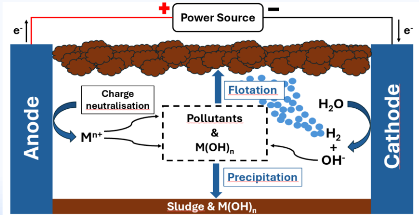
Electro-coagulation
