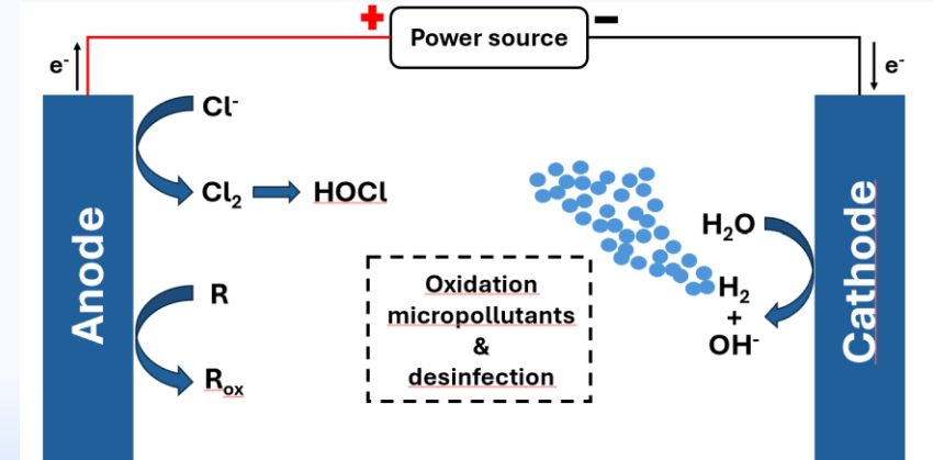
Electro-oxidation
