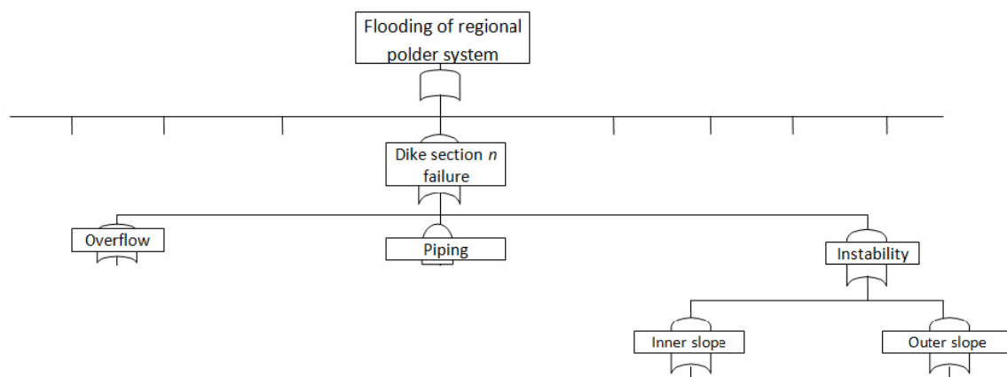
FIGURE 34 FAULT TREE FLOODING REGIONAL FLOOD DEFENCE SYSTEM
