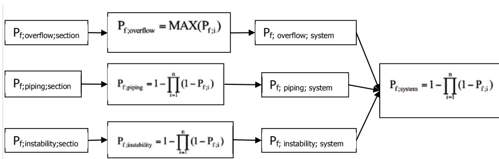
FIGURE 35 FLOW CHART METHOD OF COMBINING FAILURE PROBABILITIES
